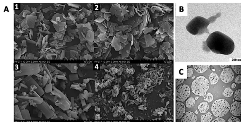
Figure 6. (A) Scanning electron microscope (SEM) images of rifampicin crystal from spray-dried samples using (1,2) ethanol, (3) methanol, and (4) water [196]. Reprinted with permission from ref. [196]. Copyright 2020 Elsevier Inc. (B) Transmission electron microscope (TEM) image of meropenem particles, scale bar: 200 nm [197]. Reprinted with permission from ref. [197]. Copyright 2020 Elsevier Inc. (C) SEM image cross-sections of Poly(lactic-co-glycolic acid) (PLGA) microspheres containing levofloxacin [198]. Reprinted with permission from ref. [198]. Copyright 2018 Elsevier Inc.
