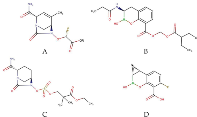
Figure 3. Chemical structures of (A) ETX0282, (B) VNRX-7145, (C) ARX-1796, and (D) QPX7728.
